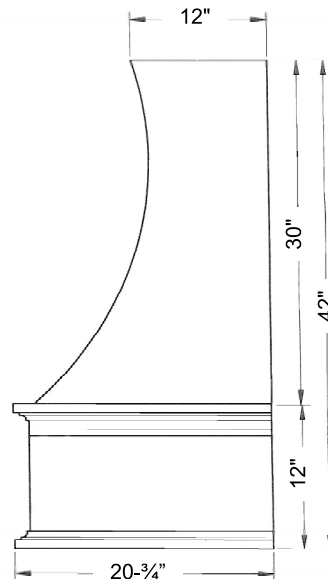
Side – Wall Hood
