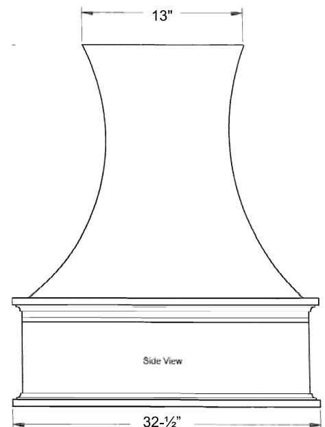
Side - Island Hood
